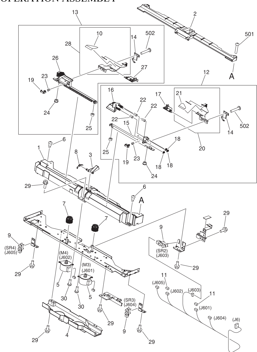
FIGURE Q30 OPERATION ASSEMBLY
