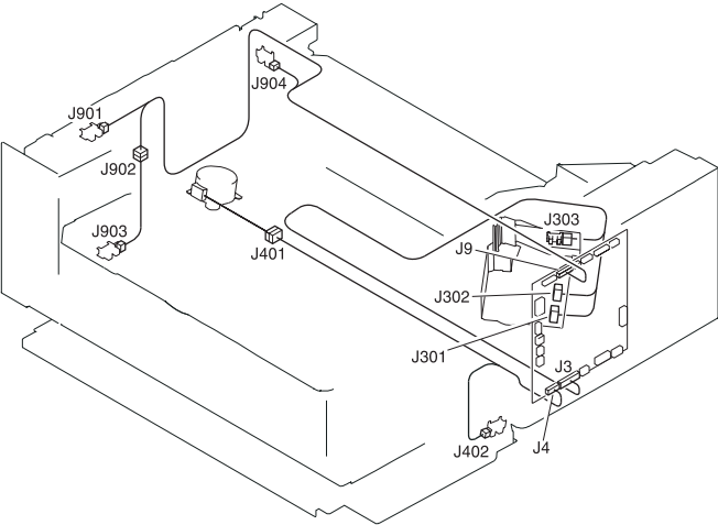
FIGURE QB LIST OF CONNECTORS
