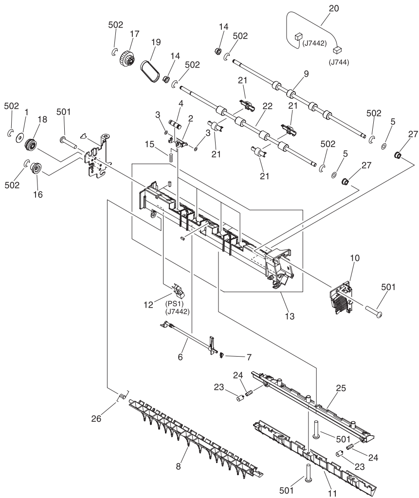
FIGURE Q38 2ND DELIVERY FRAME ASSEMBLY
