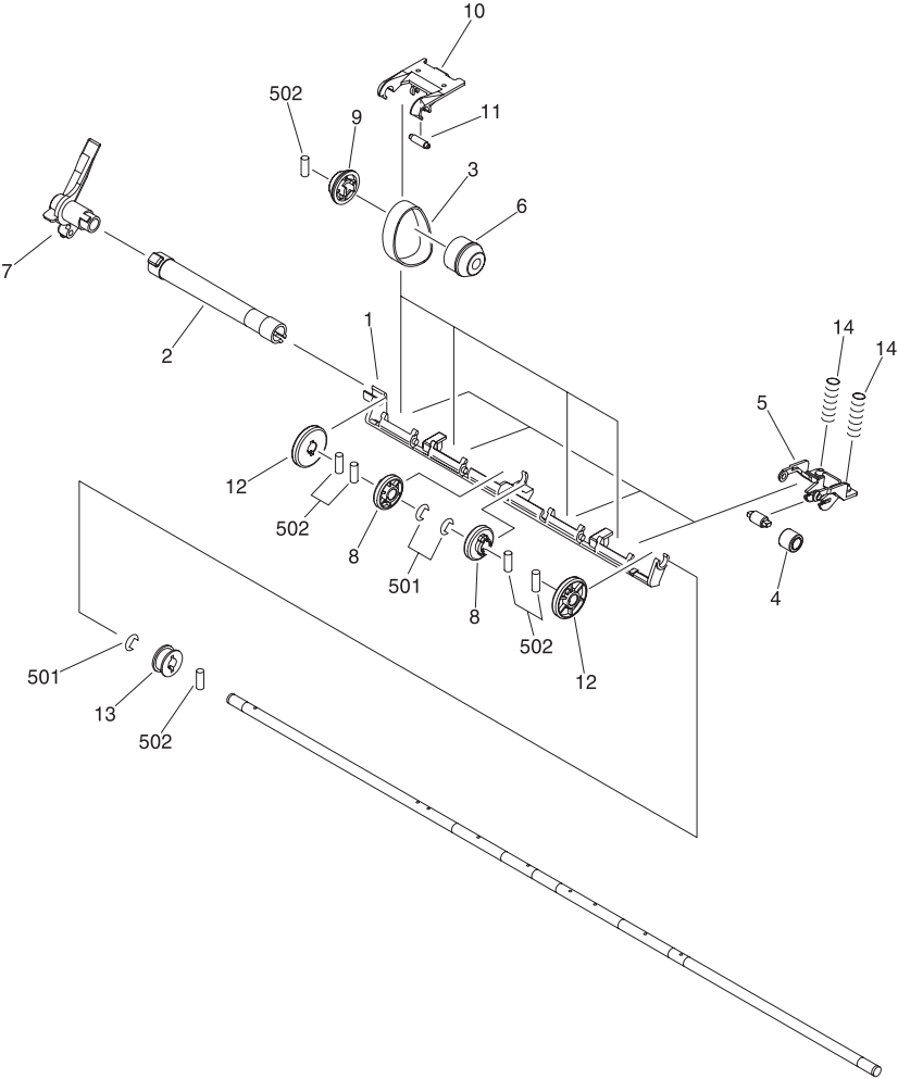
FIGURE Q31 DELIVERY ASSEMBLY
