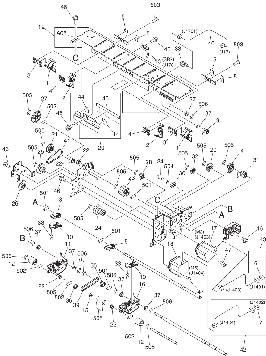
FIGURE Q32 SWING ROLLER ASSEMBLY
