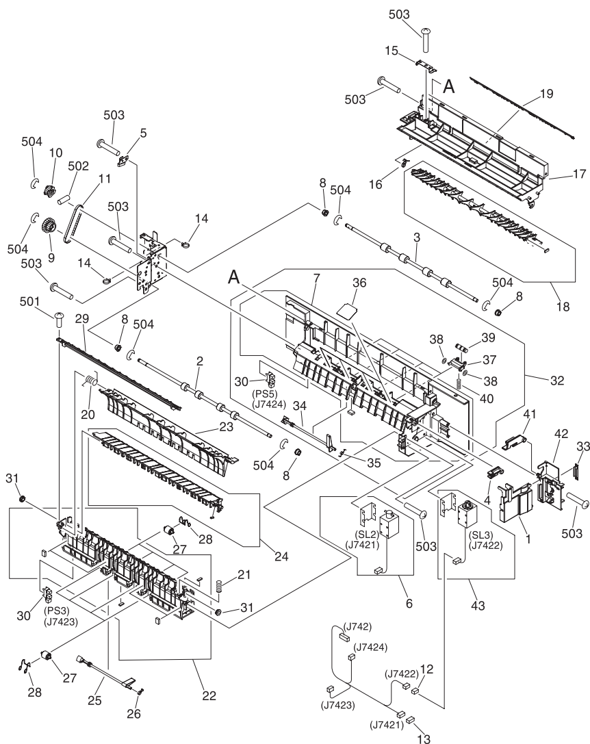
FIGURE Q39 3RD DELIVERY FRAME ASSEMBLY
