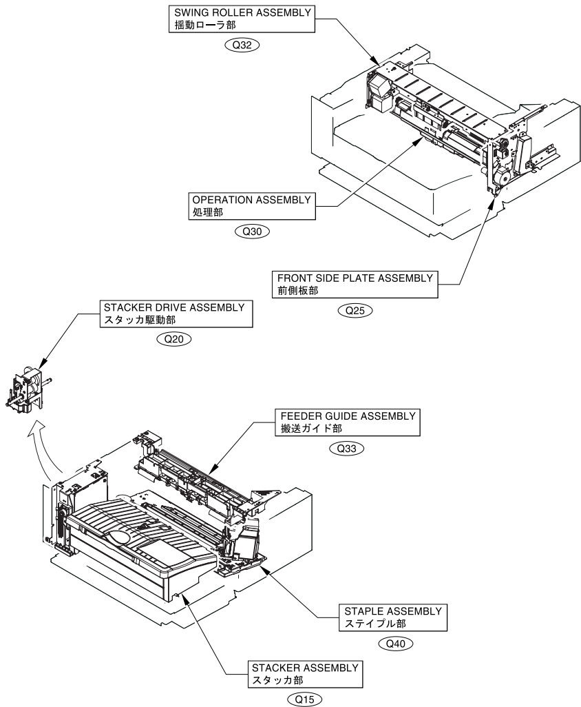
FIGURE QA ASSEMBLY LOCATION DIAGRAM
