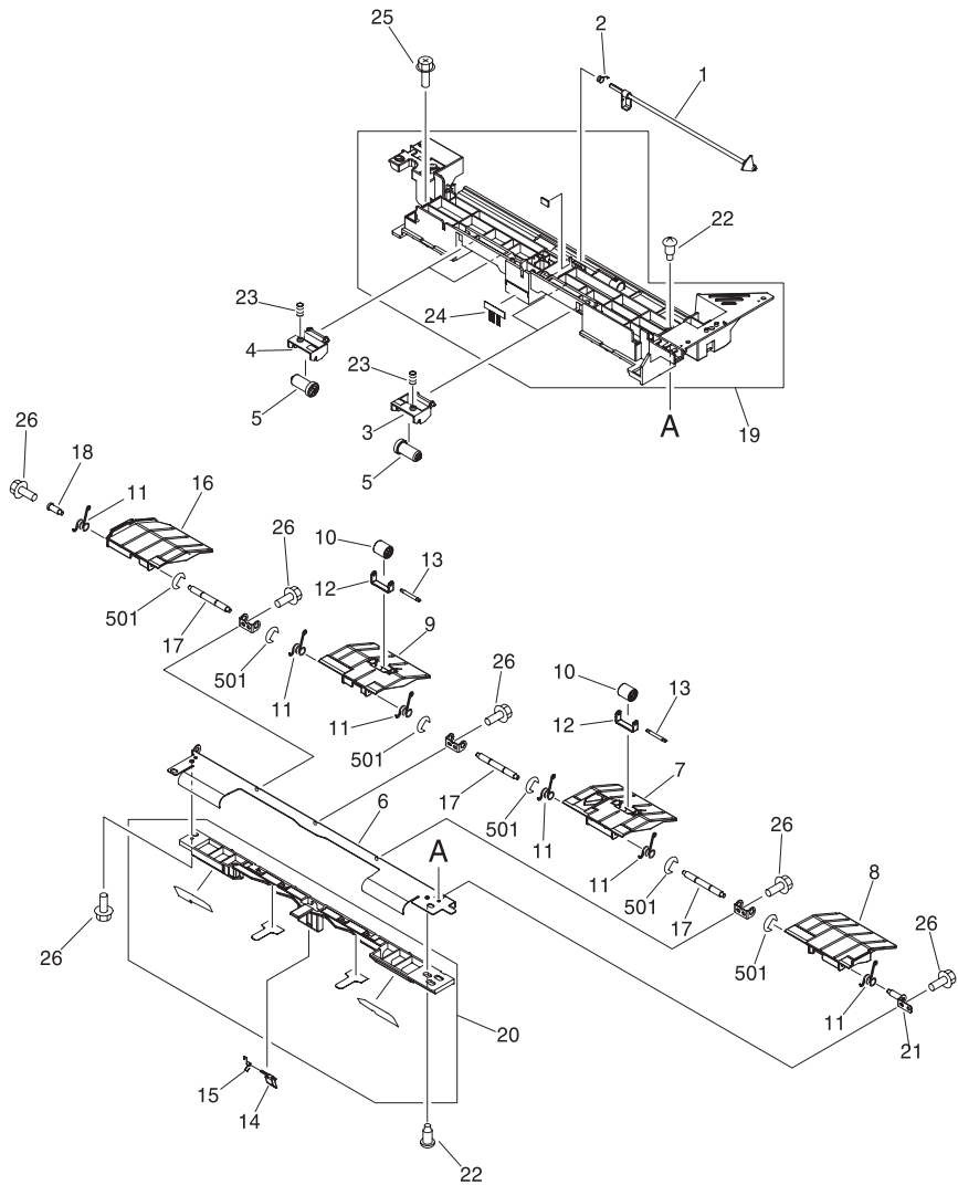
FIGURE Q33 FEEDER GUIDE ASSEMBLY
