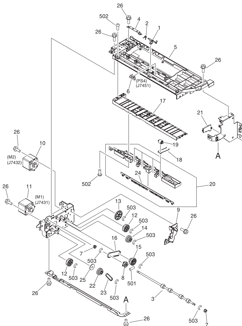
FIGURE Q37 2ND UPPER DELIVERY ASSEMBLY
