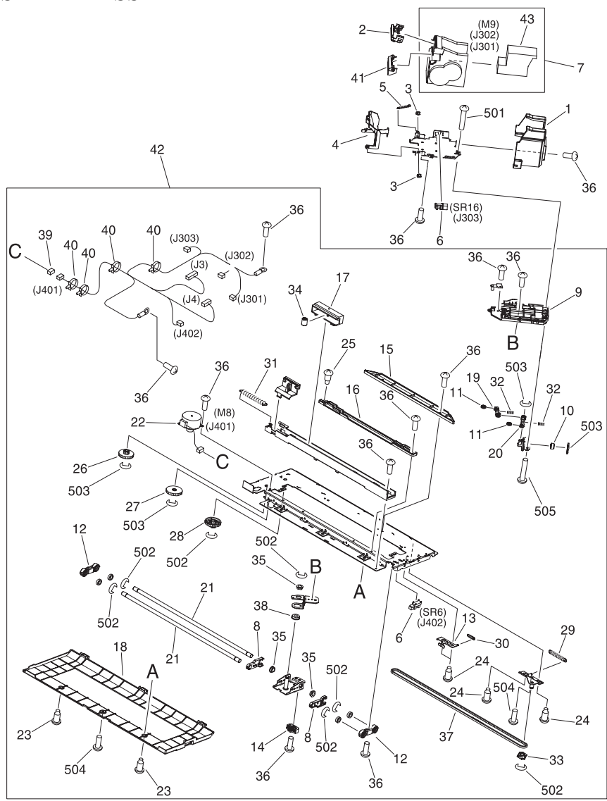
FIGURE Q40 STAPLE ASSEMBLY
